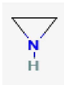
( Aziridine structure)
