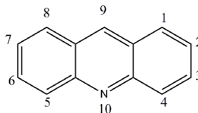
(Acridine)
