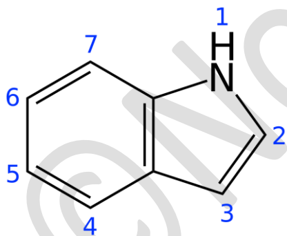
(Indole)
