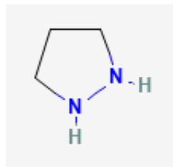
(Pyrazolidine)
